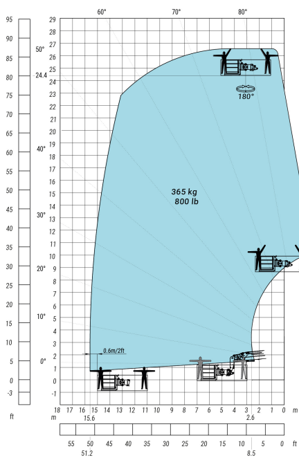
Machine on lowered stabilisers with 365 kg platform Metric
